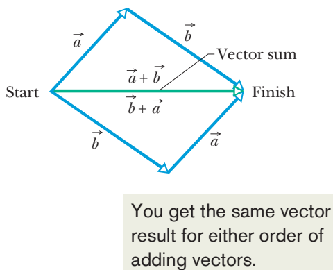
Figure 3-3 The two vectors \vec{a} and \vec{b} can be added in either order; see Eq. 3-2.
