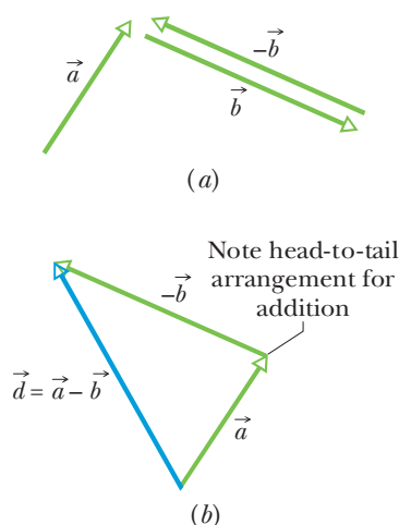
Figure 3-6 (a) Vectors \vec{a} , \vec{b} , and -\vec{b} . (b) To subtract vector \vec{b} from vector \vec{a} , add vector -\vec{b} to vector \vec{a} .
